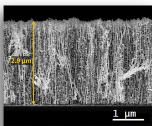
Nickel nanowires
