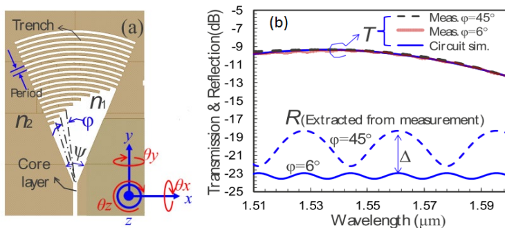
Fig.1. Example design of low back reflection grating coupler for communication-band[1].
