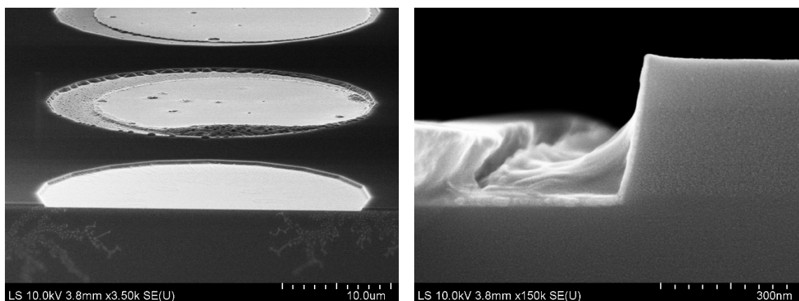
SEM images showing recessed metal bumps.
