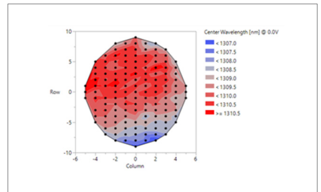
Microring Modulator Resonant Wavelength Wafer-scale distribution (300mm, 1-\sigma = 0.9\text{nm} )
