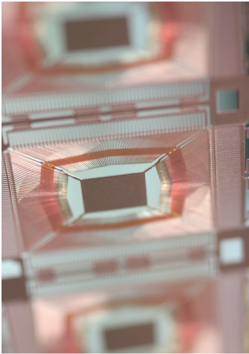
Leadframe
